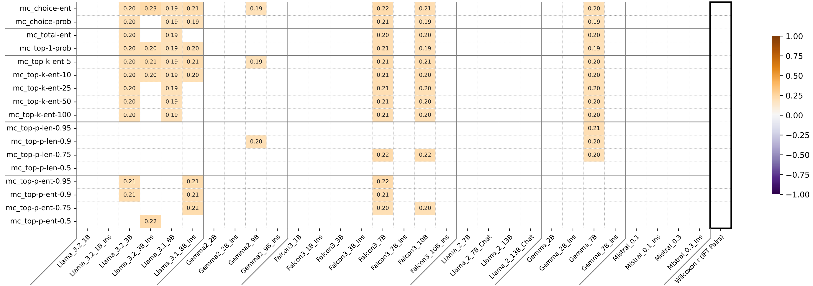
Spearman Correlation CamChoice (MCQA) human uncertainty (Human Ent) vs. model uncertainty
